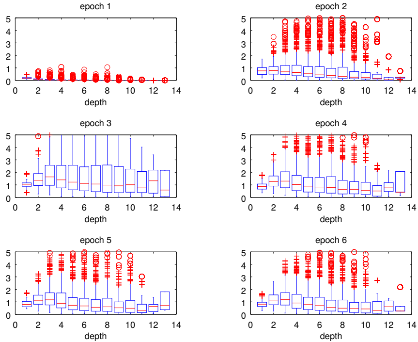
Figure 5: Ratios of norms of error vectors at keyword nodes (at different depths) to norms of error vectors at root nodes, in the RLSTM. Many gradients explode in epoch 2, but stabilize later. Gradients do not vanish, even at depth 12 and 13.
