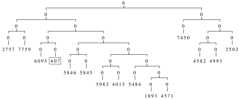
Figure 1: Example binary tree for the artificial task. The number enclosed in the box is the keyword of the sentence.
