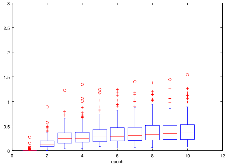
(a) RNN
