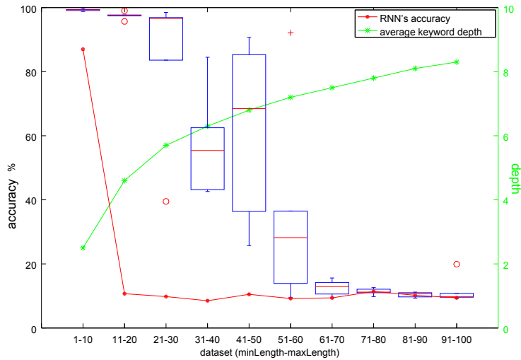
Figure 2: Test accuracies of the RNN (the best among 5 runs) and the RLSTM (boxplots) on datasets of different sentence lengths.
