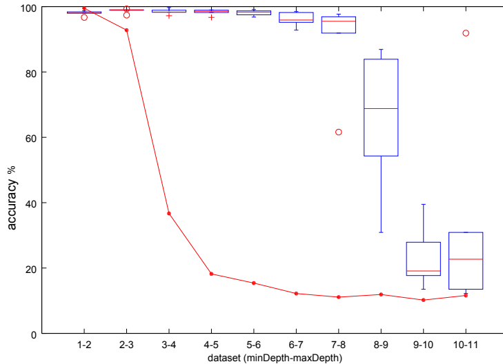
Figure 3: Test accuracies of the RNN (the best among 5 runs) and the RLSTM (boxplots) on datasets of different keyword depths.
