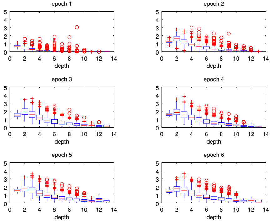
Figure 4: Ratios of norms of error vectors at keyword nodes to norms of error vectors at root nodes w.r.t. the keyword node depth in each epoch of training the RNN. Gradients gradually vanish with greater depth.
